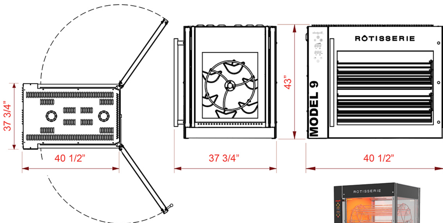
TOP VIEW
